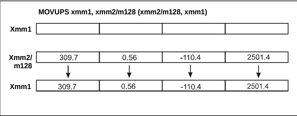
Figure 3-49. Operation of the MOVUPS Instruction
