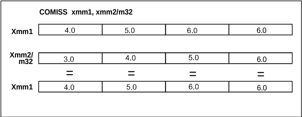
Figure 3-26. Operation of the COMISS Instruction, Condition Four
