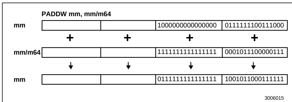
Figure 3-55. Operation of the PADDW Instruction
