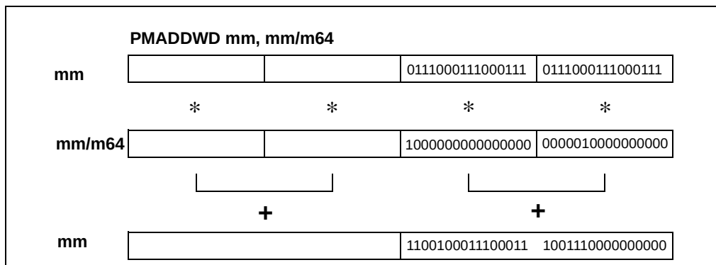
Figure 3-65. Operation of the PMADDWD Instruction
