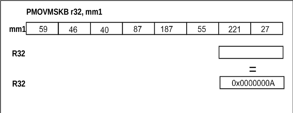
Figure 3-70. Operation of the PMOVMASKB Instruction
