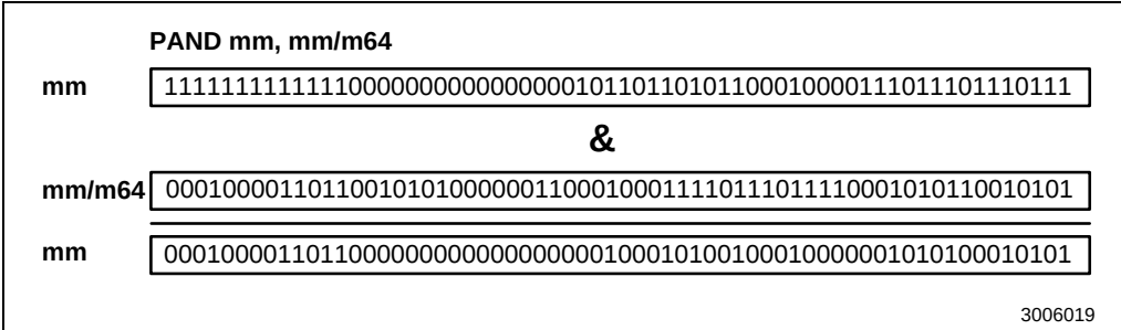
Figure 3-58. Operation of the PAND Instruction
