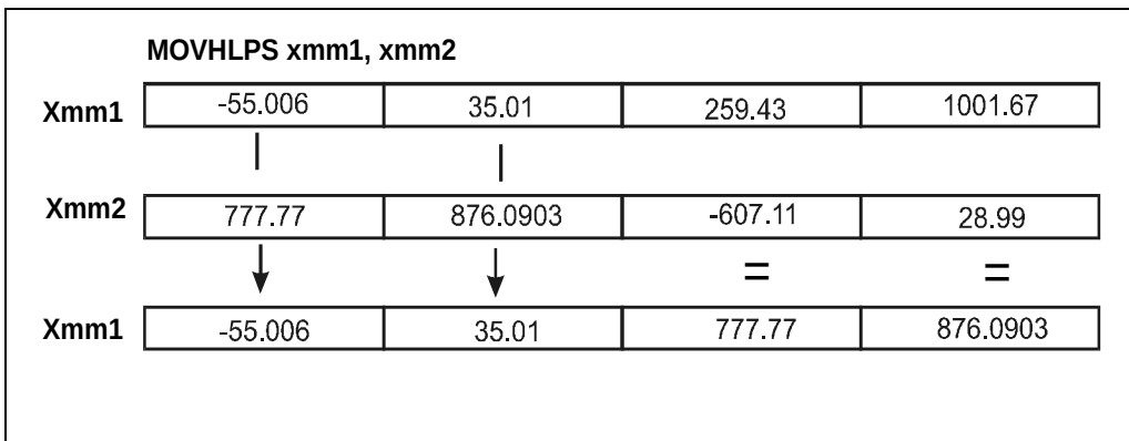
Figure 3-42. Operation of the MOVHLPS Instruction
