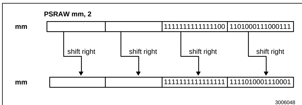
Figure 3-78. Operation of the PSRAW Instruction
