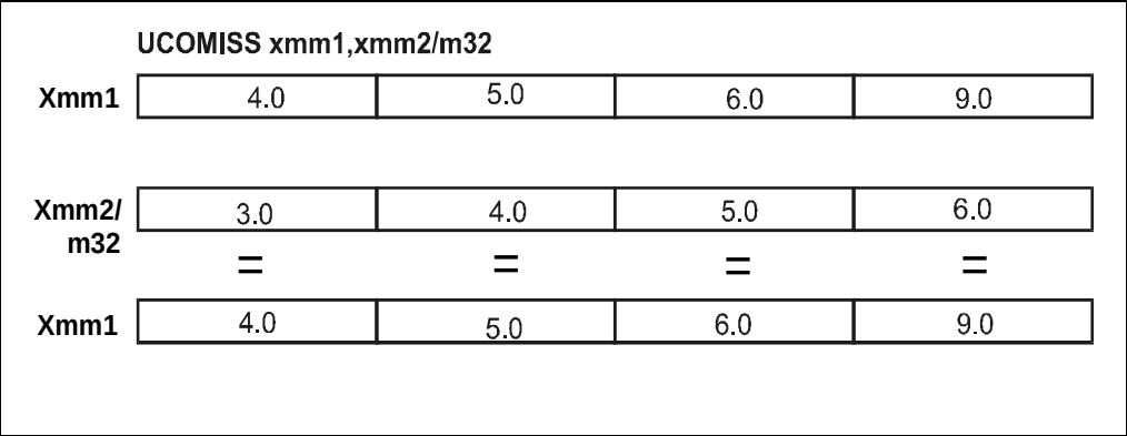
Figure 3-96. Operation of the UCOMISS Instruction, Condition Two
