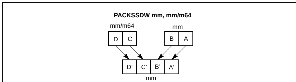
Figure 3-53. Operation of the PACKSSDW Instruction
