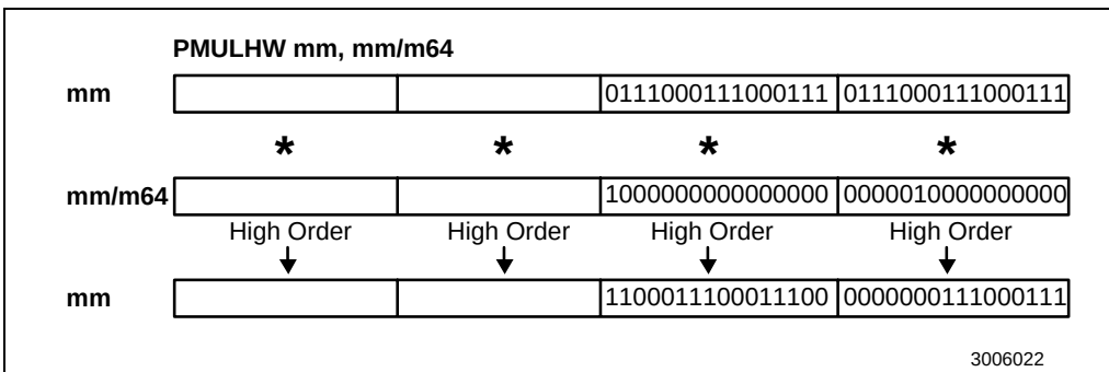
Figure 3-72. Operation of the PMULHW Instruction
