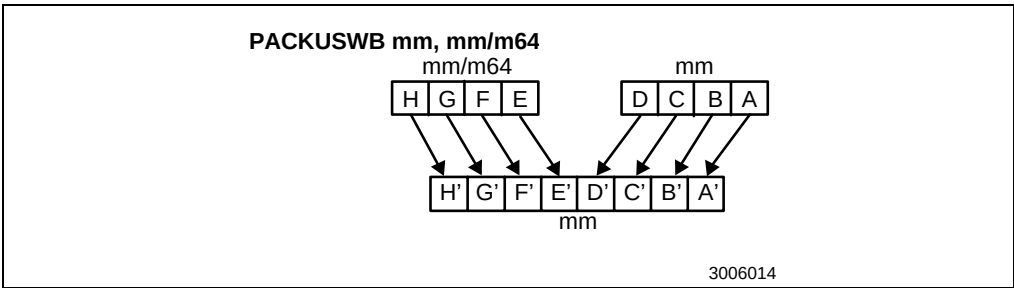
Figure 3-54. Operation of the PACKUSWB Instruction
