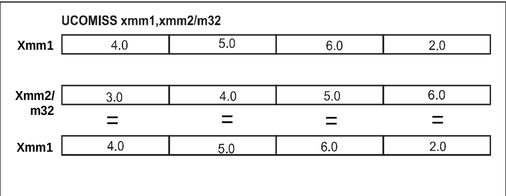
Figure 3-97. Operation of the UCOMISS Instruction, Condition Three
