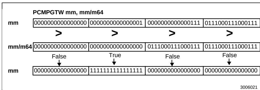
Figure 3-62. Operation of the PCMPGTW Instruction
