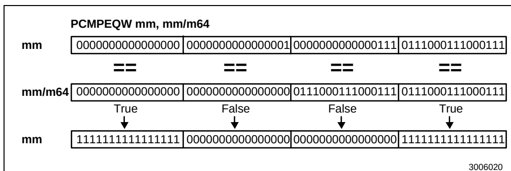
Figure 3-61. Operation of the PCMPEQW Instruction
