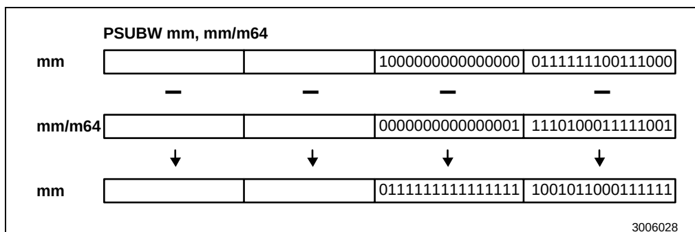
Figure 3-80. Operation of the PSUBW Instruction
