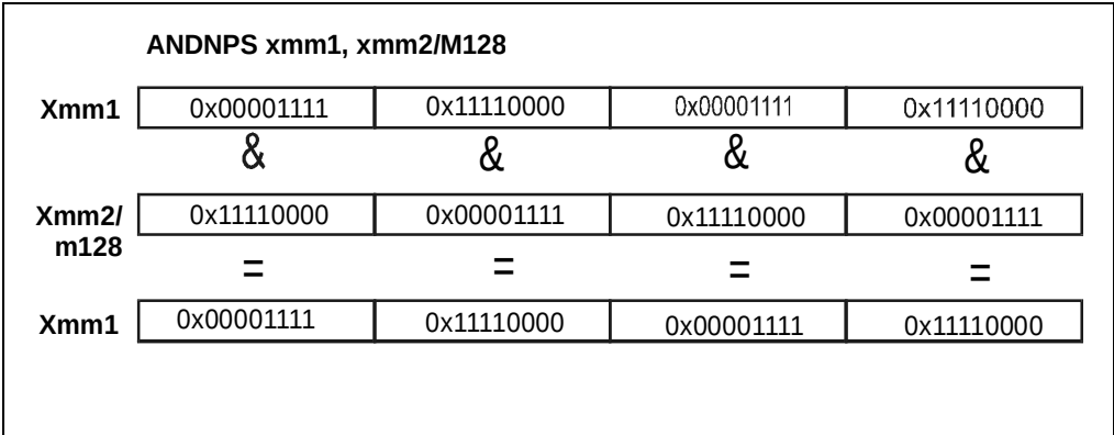
Figure 3-5. Operation of the ANDNPS Instruction
